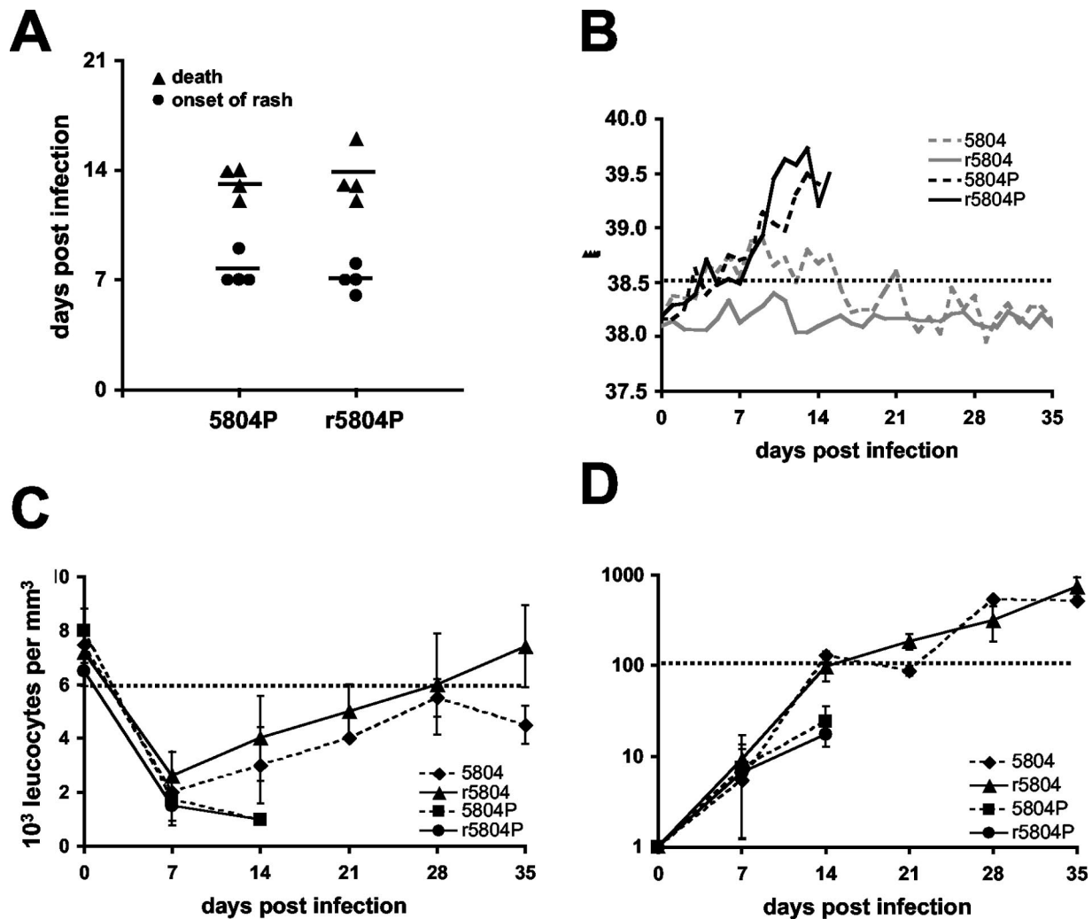
FIG. 4. Course of disease in animals infected with parental or recombinant, attenuated or virulent viruses. (A) Comparison of disease progression in animals infected with the original (5804P) or recombinant (r5804P) virulent strains. Onset of rash is indicated by dots, and time of death is indicated by triangles. Each pair of symbols represents one animal. (B) Rectal temperatures of animals infected with the different attenuated or virulent strains (5804, n = 2 ; r5804, n = 4 ; 5804P, n = 4 ; r5804P, n = 4 ). Temperatures were recorded daily. The temperature ( 38.5^{\circ}\text{C} ) above which animals were considered to be pyrexemic is indicated by a dotted line. Gray lines are used for attenuated viruses, and black lines are used for the pathogenic strains. Interrupted lines are used for the parental viruses, and continuous lines are used for strains recovered from infectious cDNA. Mean values are indicated. Leukocyte count (C) and neutralizing antibody titer (D) of animals infected with the different viruses (same animals as described in panel B) are shown. Blood samples were taken at the indicated time points. Lines are drawn with the same conventions as those used for panel B. Error bars are included for each data point. The leukocyte concentration ( 6,000 cells per \text{mm}^3 ) below which animals are considered leukopenic and the protective neutralizing antibody titer ( \geq 100 ) are indicated by a dotted line in panels C and D, respectively.
